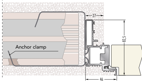
Frame on solid wall
