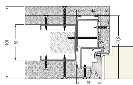
Frame on stud wall with two plasterboards Finished wall thickness 100 mm
