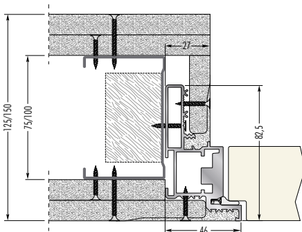
Frame on stud wall with two plasterboards Finished wall thickness 125/150 mm
