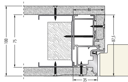
Frame on solid wall with one plasterboard Finished wall thickness 100 mm
